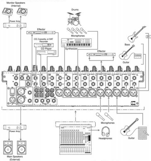
Example of Speaker Arrangement
